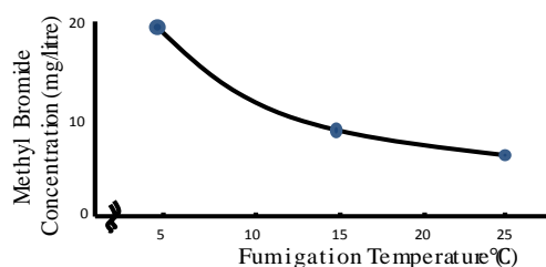
Figure 2. Effects of temperature on Methyl Bromide dose required to achieve LC99 after 24hrs fumigation.
