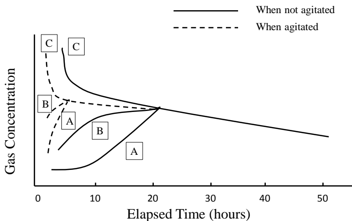
Figure 3. Gas diffusion in a fumigation chamber over time: A-Upper, B-Middle, and C-Lower chamber gas probes
