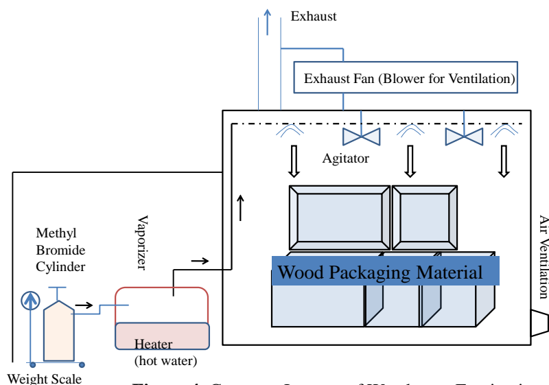
Figure 4. Common Layout of Warehouse Fumigation
