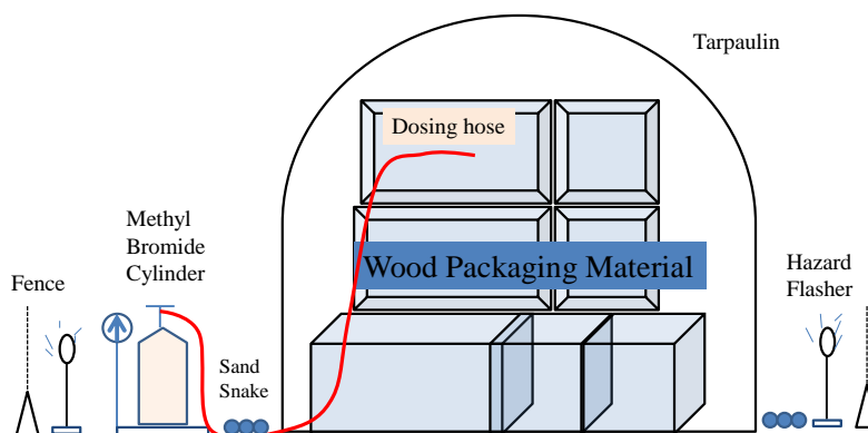
Figure 5. Common Layout of Tarpaulin Fumigation
