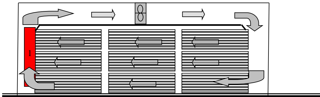
Figure 3: A heating chamber in which the heating pipes are located with a fan above the wood stack. The cold spot is likely to be nearest the exit side of the stack and the temperature sensor should be placed where the air exits the wood stack (marked “1”).
